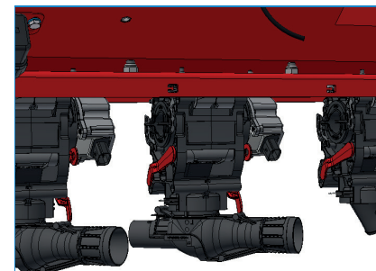
FertiSmart Fertiliser Unit With MSM (Monosem Smart Motors) drive One motor per dosing unit
